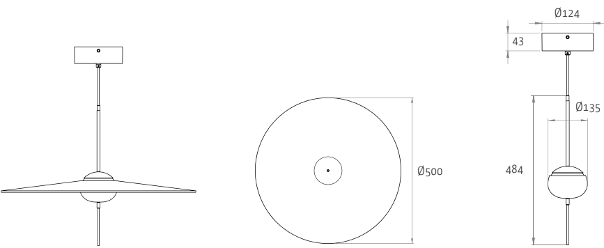
MODEL L500, shade 500 mm, body L
