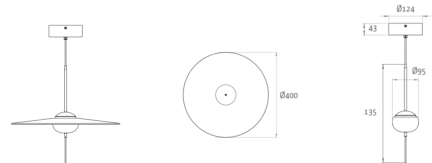
MODEL M400, shade 400 mm, body M
