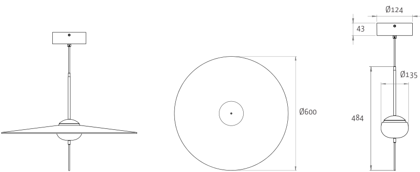
MODEL L600, shade 600 mm, body L
